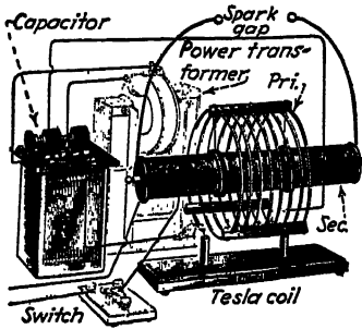
Tesla coil with associated apparatus.
